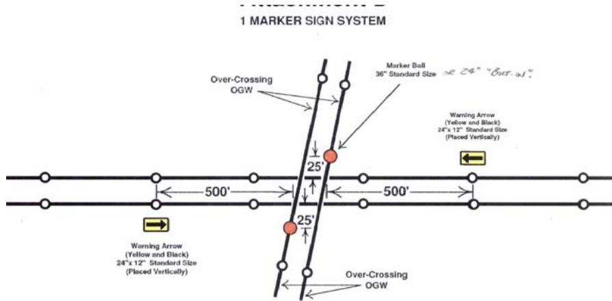
Transmission Line Over-Crossing Marking Diagram
