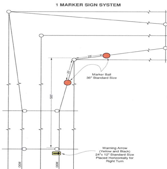
Transmission Line Horizontal Angle (turns 45° and greater) Marking Diagram
