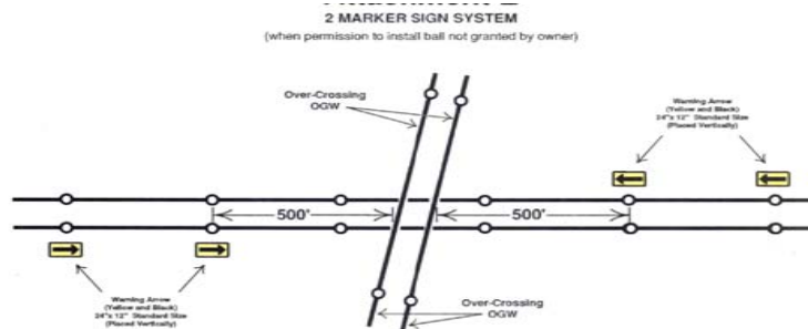
Transmission Line Over-Crossing Marking Diagram
